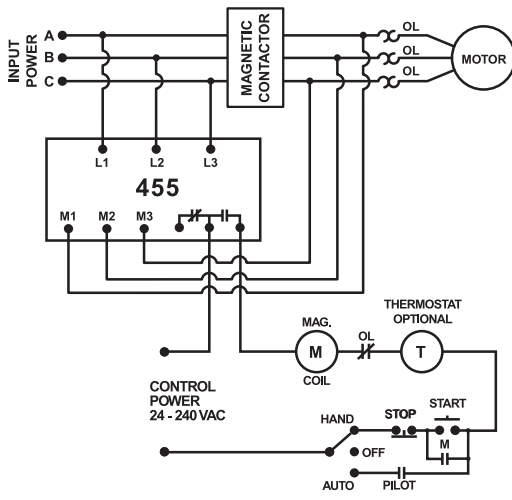
MODEL 455 WITH MOTOR CONTROL USING A 3-POLE CONTACTOR
